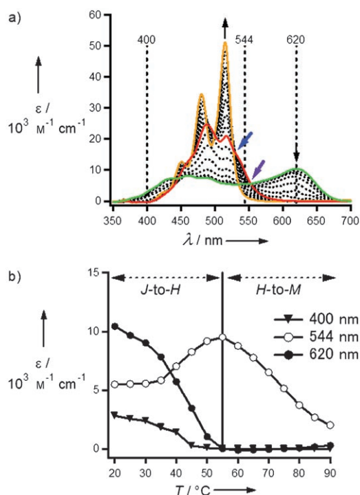
Figure 3. a) Temperature-dependent UV/Vis spectra of 1 /dCA = 1:1 mixture in MCH ( c=1.4 \times 10^{-5} M). The spectra at 20, 55, and 90 °C are shown as green, red, and yellow lines, respectively. Black arrows indicate spectral changes upon increasing temperature. Purple and blue arrows point to the isosbestic points in the first (20–55 °C, 554 nm) and the second transitions (60–90 °C, 523 nm), respectively. b) Plot of \epsilon at 400 (▼), 544 (○) and 620 nm (●) versus temperature.
