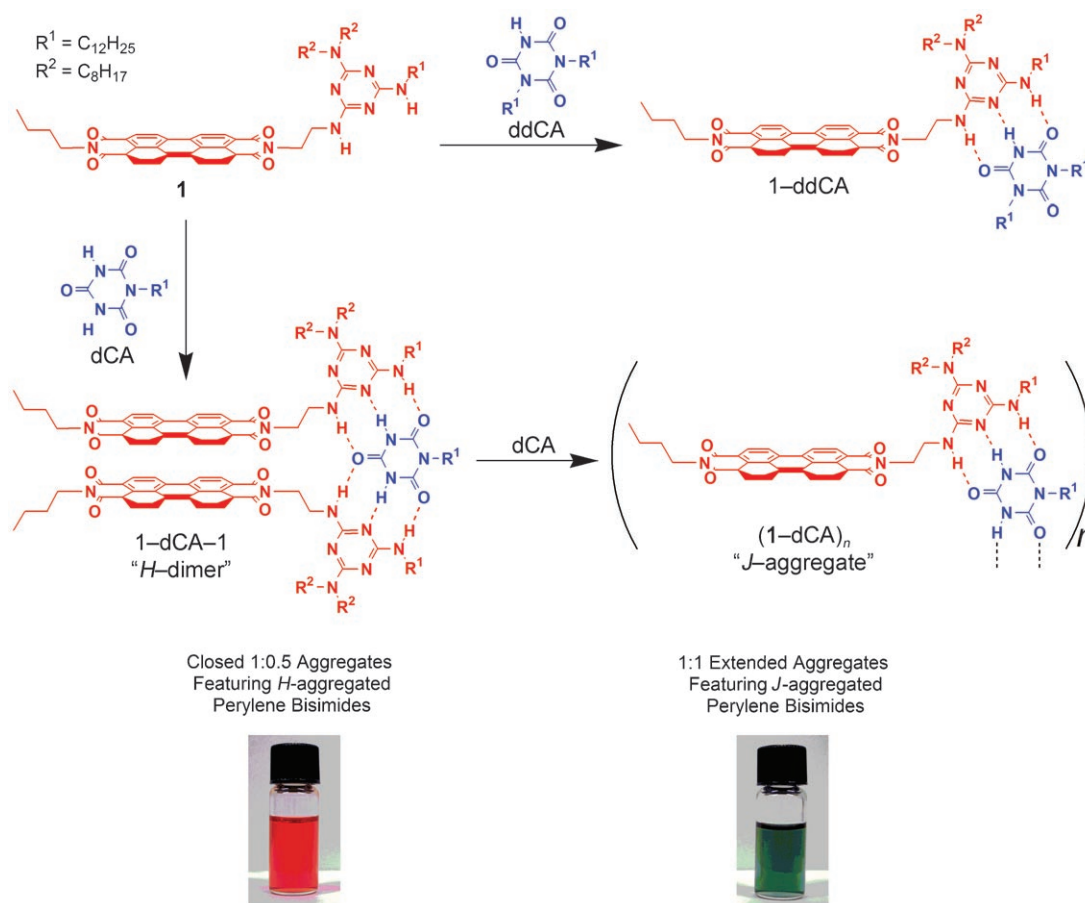
Figure 1. Complexation of 1 with the monotopic cyanurate ddCA and the ditopic cyanurate dCA. For 1:0.5 and 1:1 aggregates of 1 and dCA, photographs of their methylocyclohexane solutions are shown.
