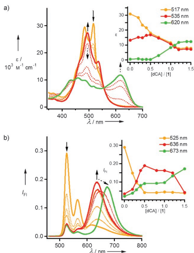
Figure 2. a) UV/Vis and b) fluorescence ( \lambda_{\text{ex}}=450 nm) titration experiments of 1 ( c=1.4 \times 10^{-5} M) with dCA. Yellow, red, and green solid curves are the spectra at 1 /dCA = 1:0, 1:0.5, and 1:1.2 (UV/Vis) or 1:1.5 (fluorescence), respectively. Solid and dashed arrows indicate the transitions from yellow to red and red to green spectra, respectively. Insets show changes of \epsilon and fluorescence intensities at several wavelengths.
